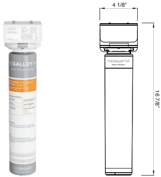
Water Filtration System
