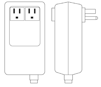
Appliance Control Box 4 3/8"H x 3"W x 1 3/4"D 120v 15Amp 1Hp
