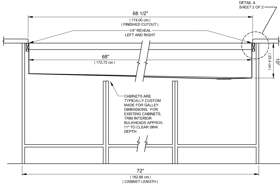
INSET CABINET INSTALLATION AND COUNTER TOP CUTOUT DETAIL SHEET 1 OF 2
